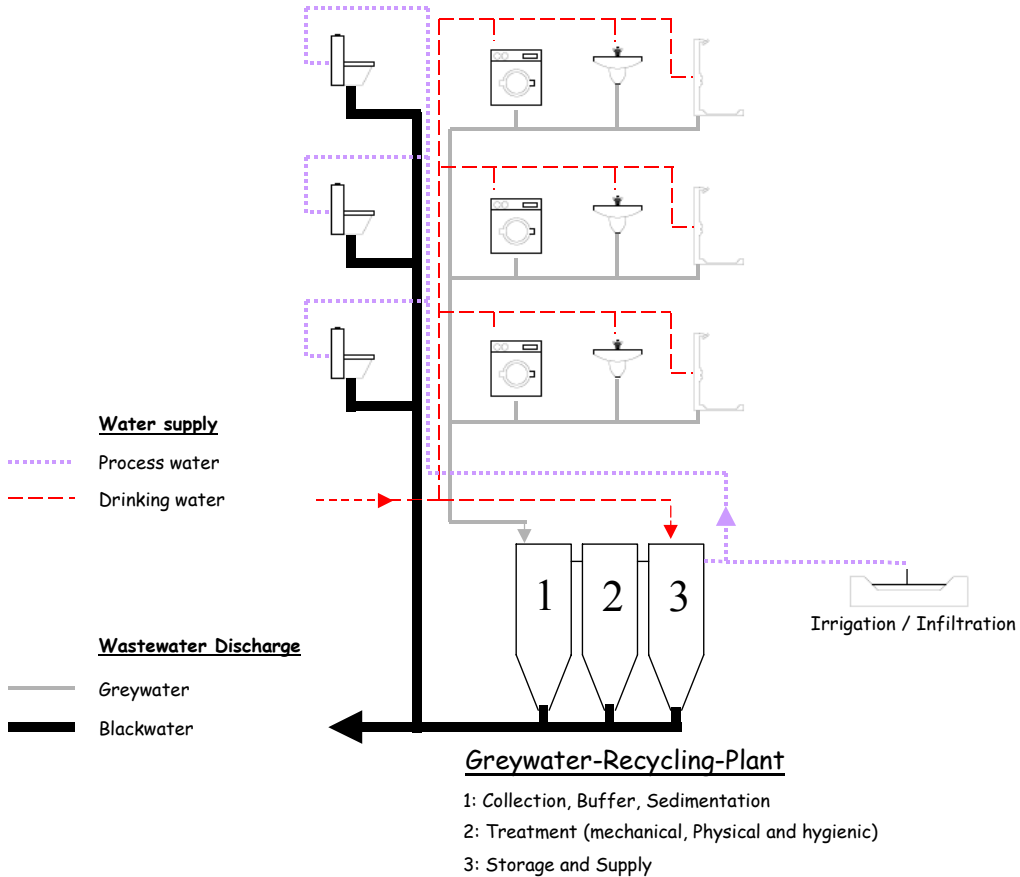
Figure 2: Typical application of greywater recycling from several households (Note: As an alternative, a drinking water connection to the washing machine is offered to the tenant).
